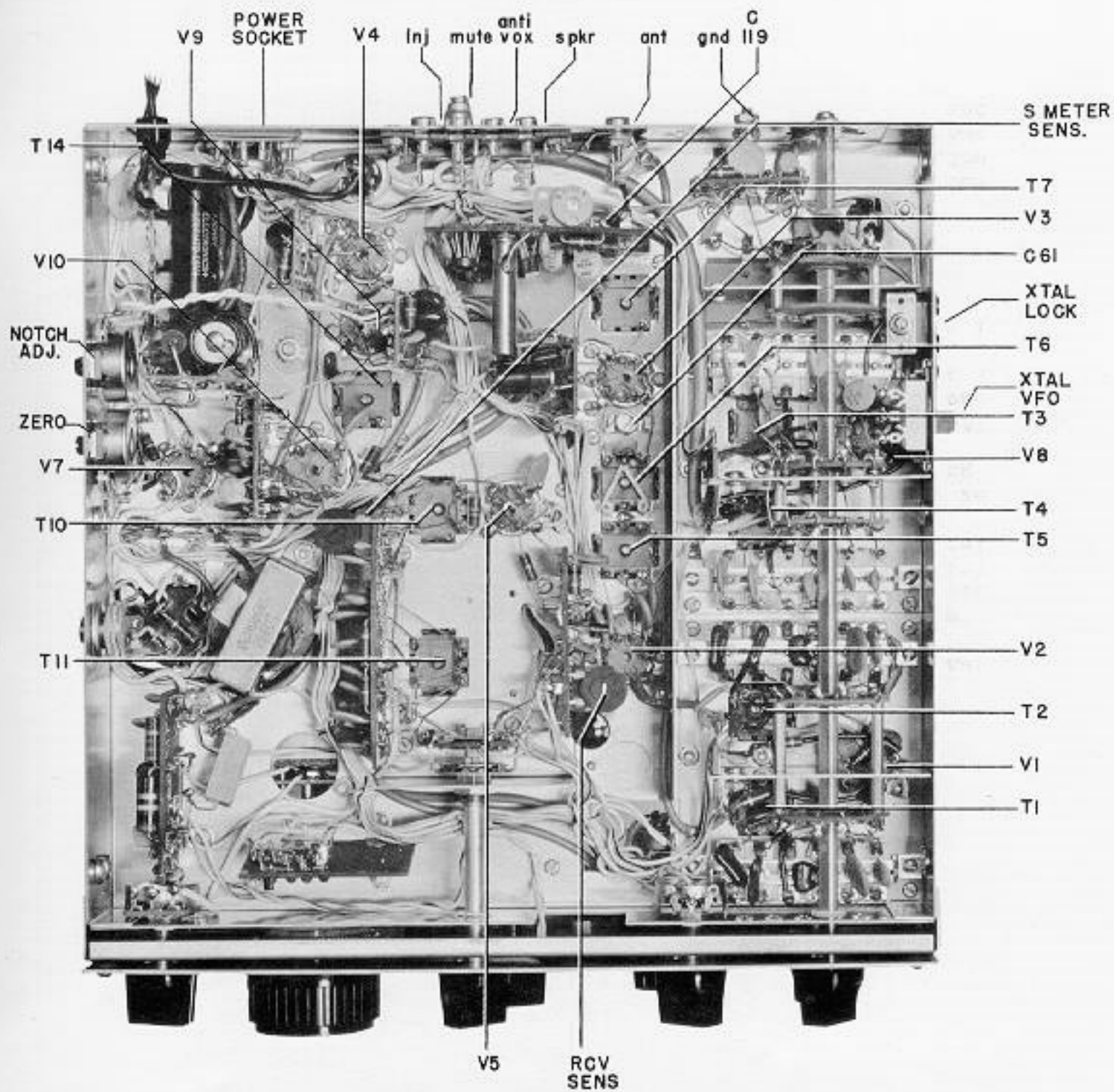
FIGURE #13 BOTTOM VIEW
