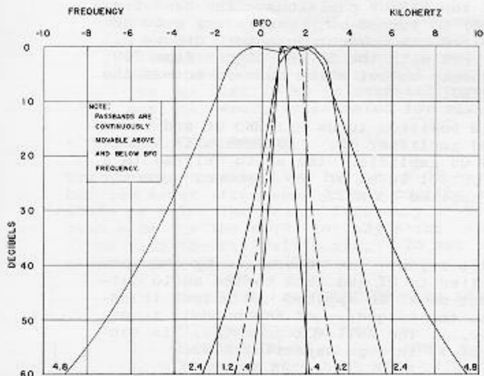
FIGURE #7 — SELECTIVITY CURVES
